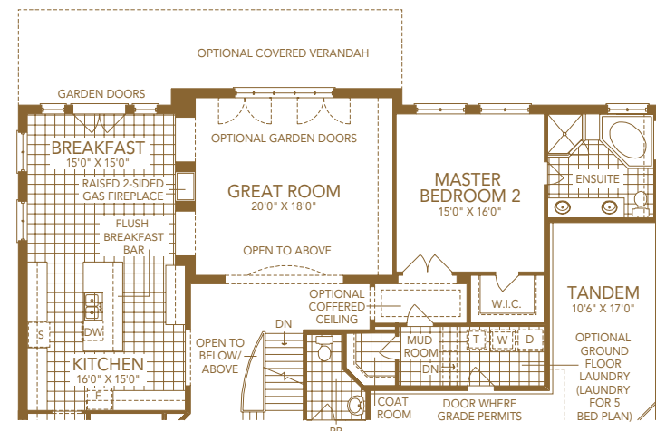
PART. OPT. MAIN FLOOR PLAN ELEVATION A
